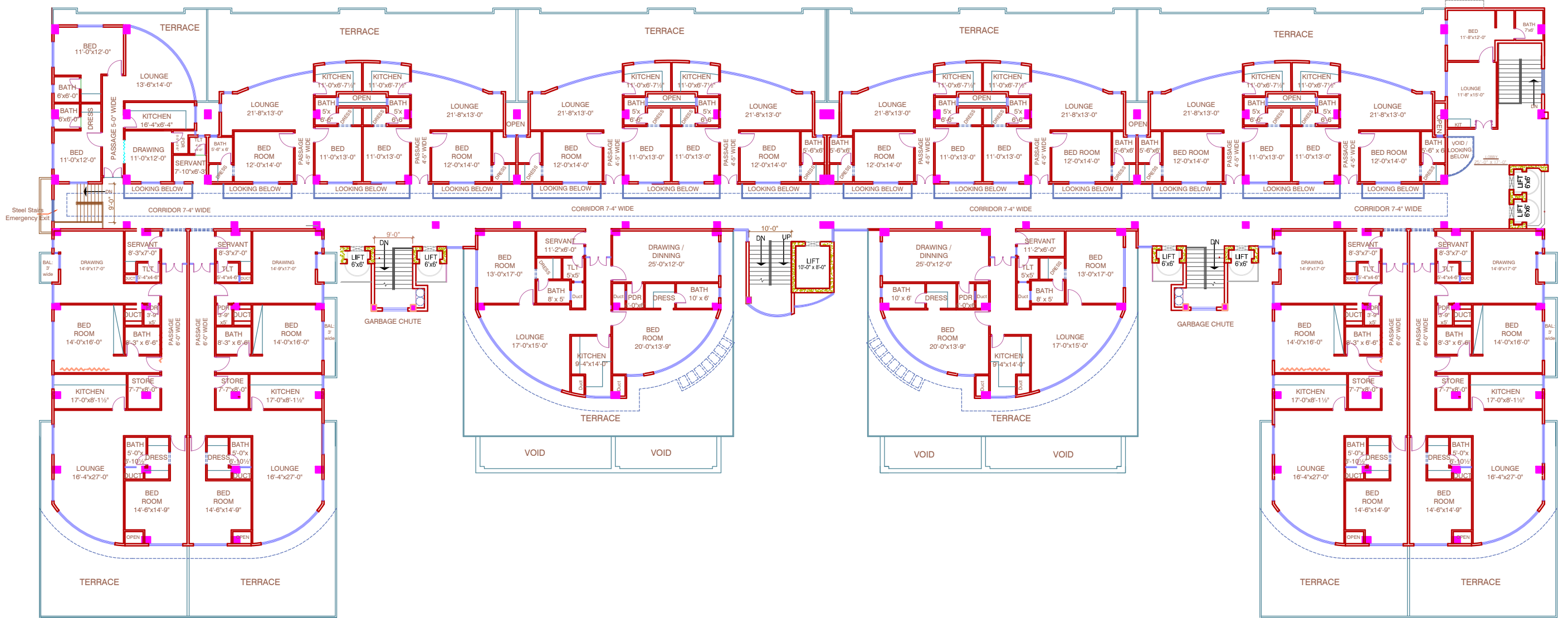
EIGHTH FLOOR PLAN
